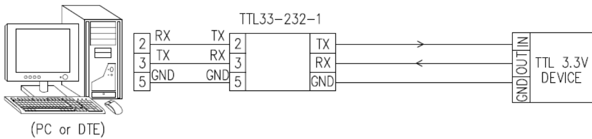
FIGURE 1: TTL33-232-1 CONNECTION DIAGRAM
